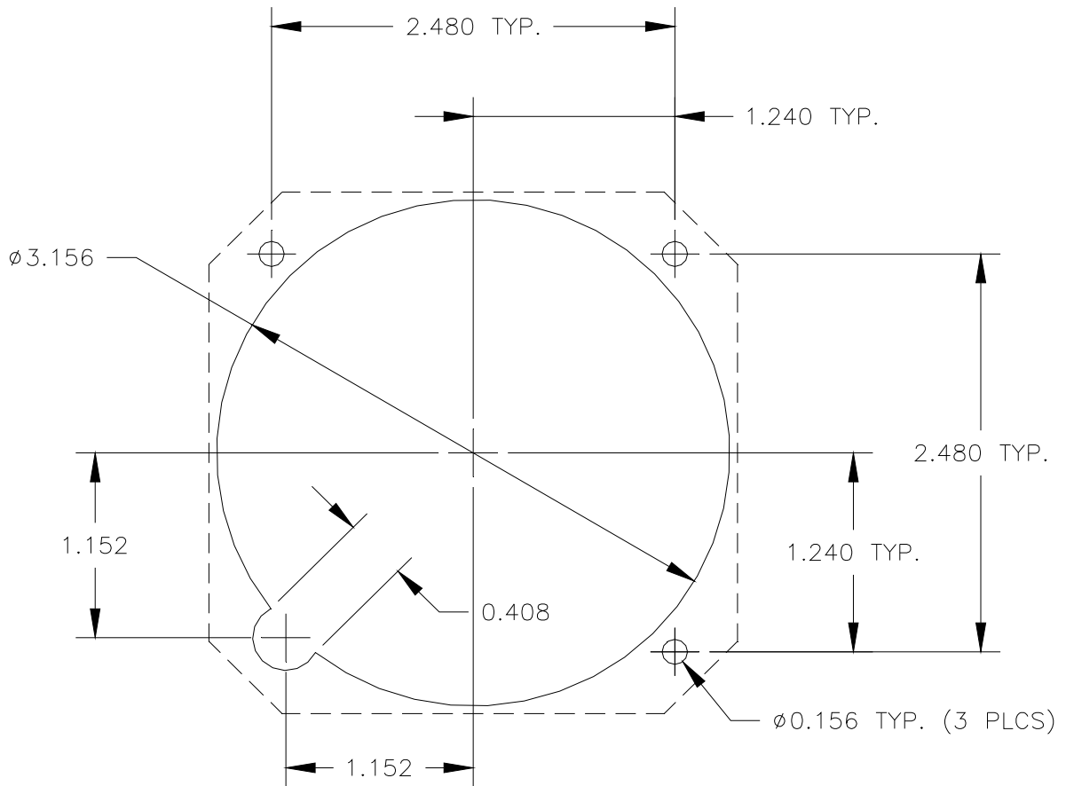
FIGURE 3-2 CUTOUT DIMENSIONS FOR PANEL MOUNTING
