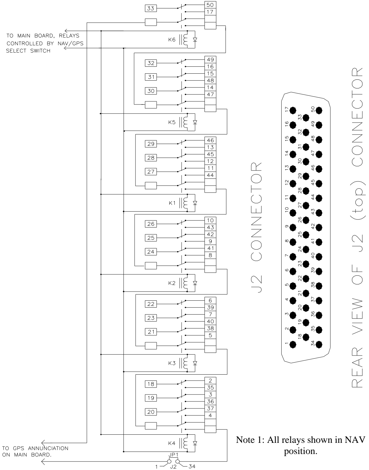
FIGURE 3-2 SCHEMATIC PINOUT, 50 PIN DSUB
