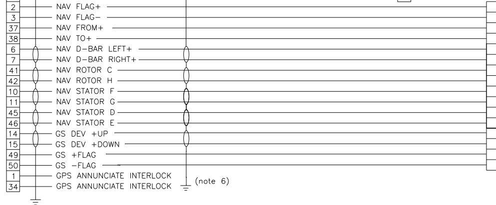
FIGURE 3-5 WIRING DIAGRAM, MD41-924A/934A KLN 900 (14V)
