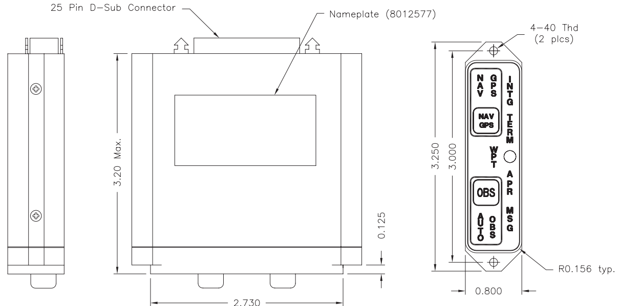
Vertical Mount
