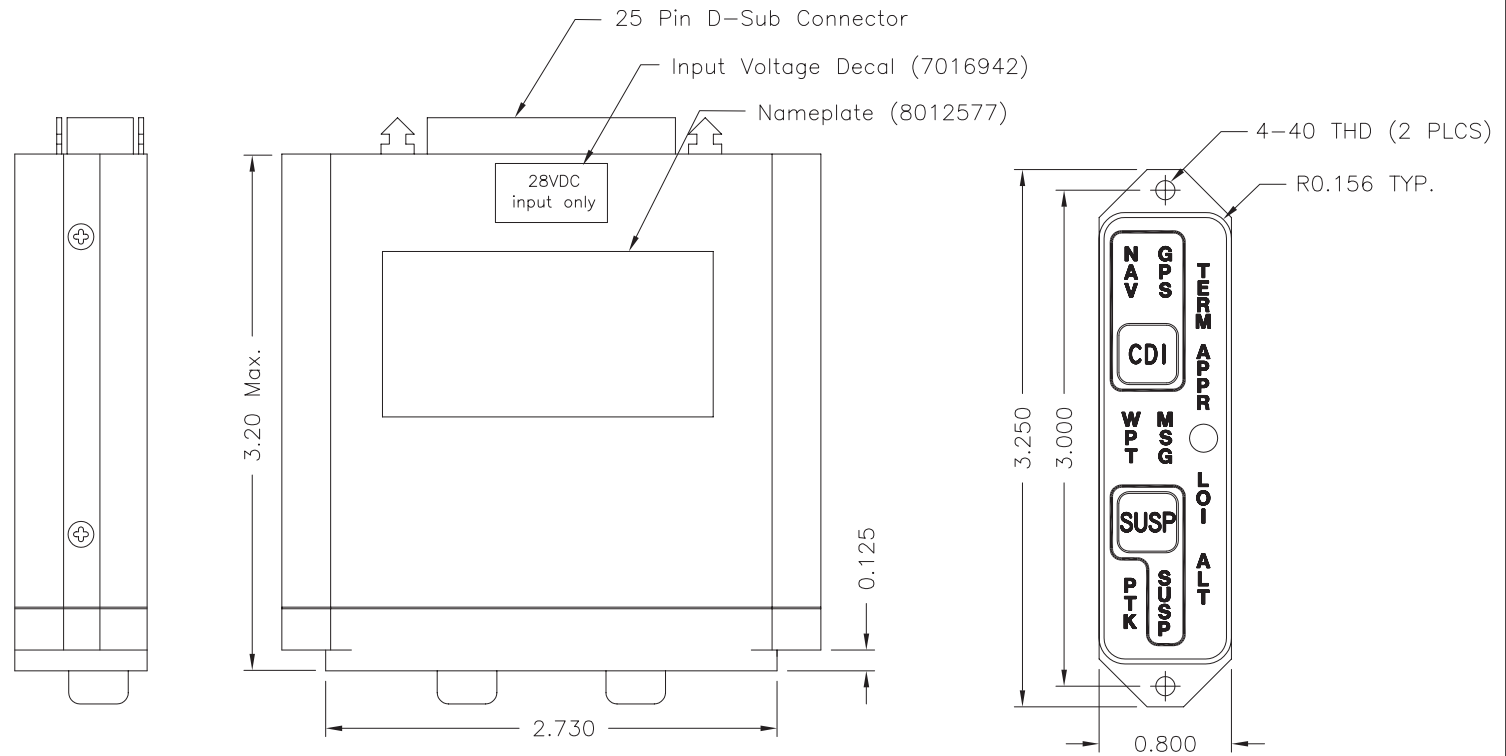
Vertical Mount
