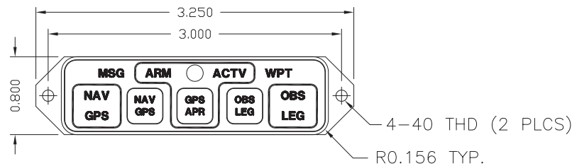
Horizontal Mount
