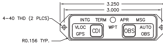
Horizontal Mount
