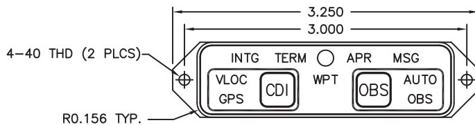
Horizontal Mount
