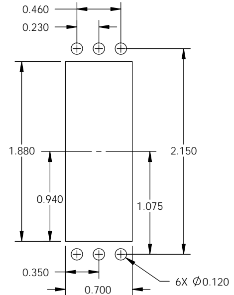
Panel Cutout
