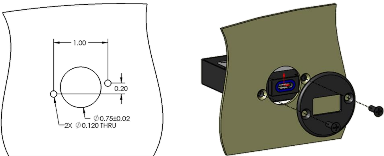
Figure 3.8 Single Port Rear Mount Circular Faceplate
