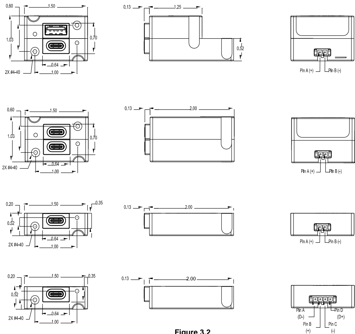
Figure 3.2 TA360 Outline Drawing
