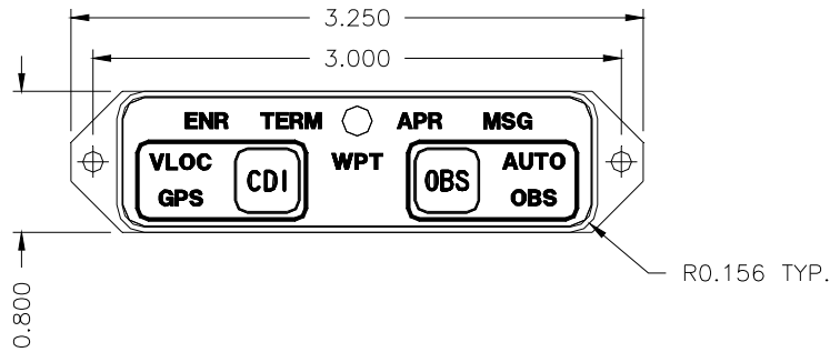
HORIZONTAL MOUNT MD146X
