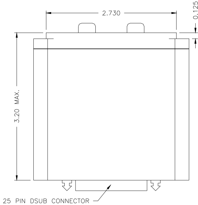
HORIZONTAL MOUNT MD146X
