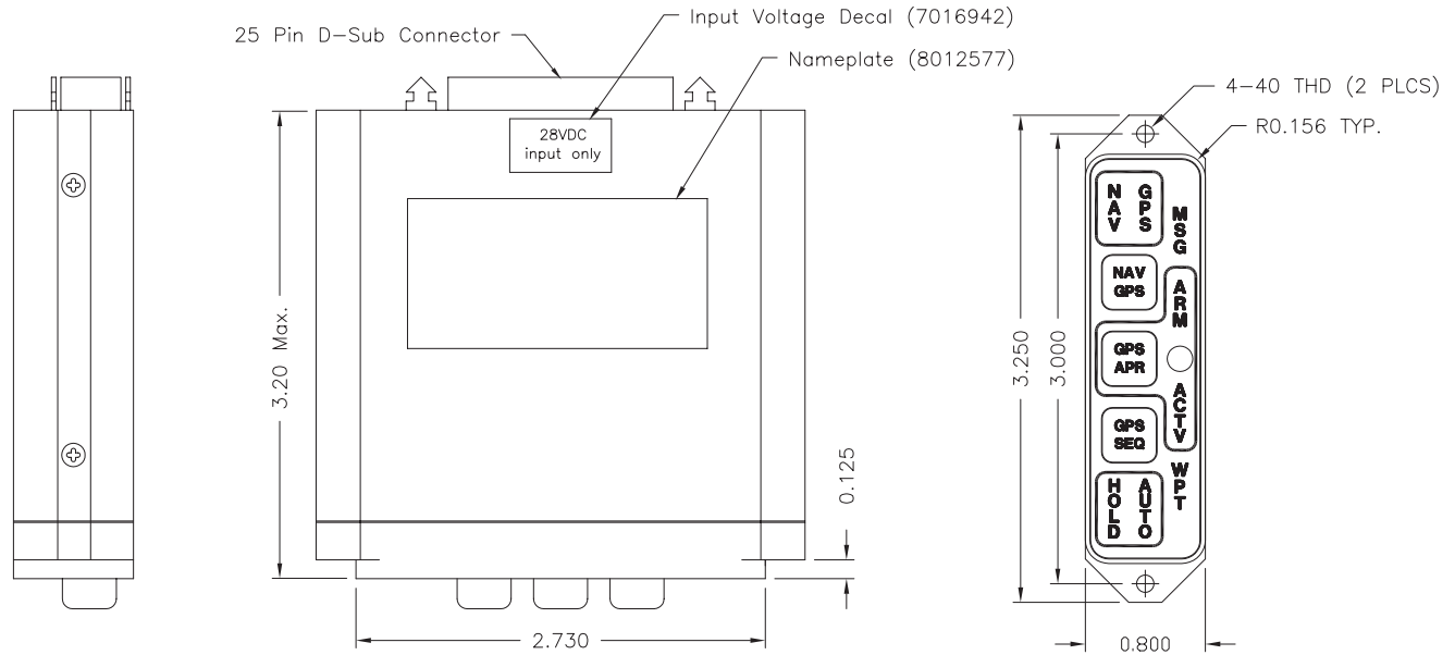
Vertical Mount
